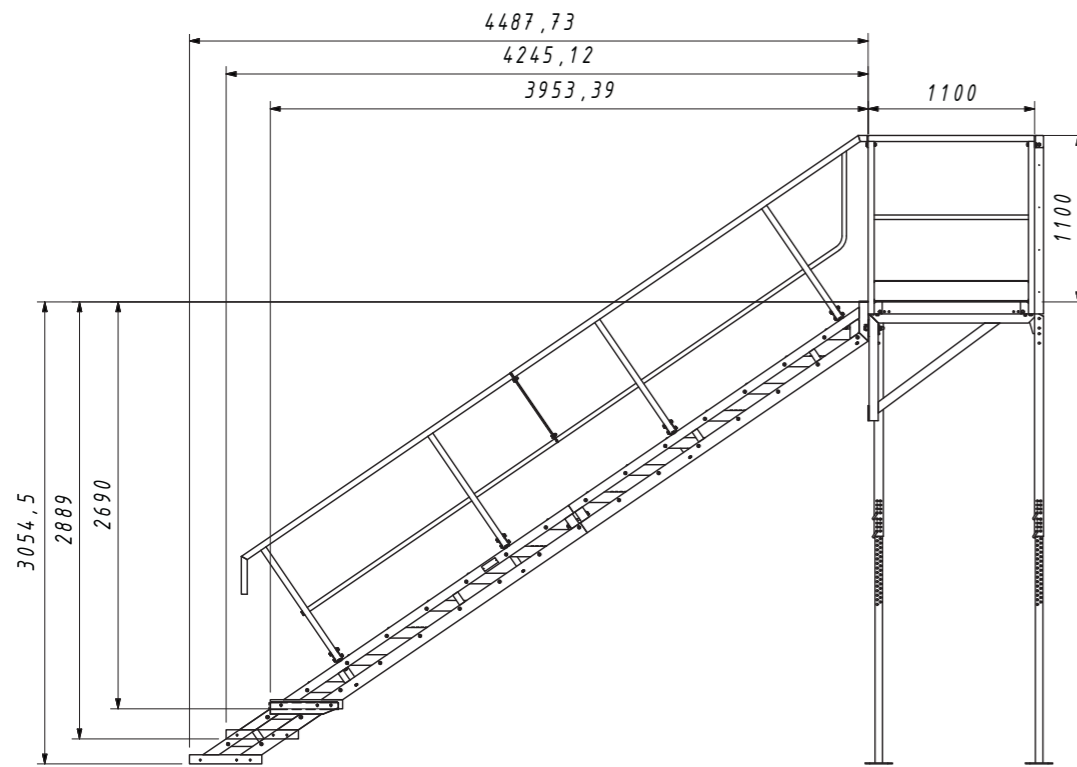
VAR3 Railing 1.1 Industrial type
